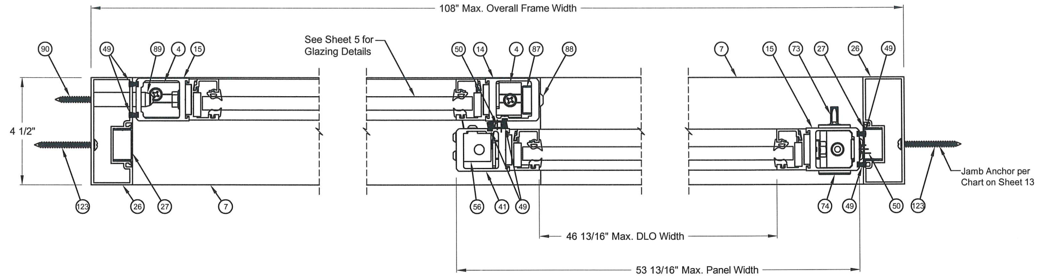
Section F-F, Narrow Stile SINGLE SLIDE FIXED SIDELITE SHOWN
