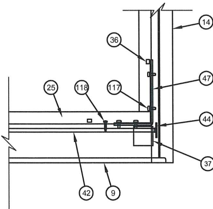
Sidelite Bottom Lead Corner
