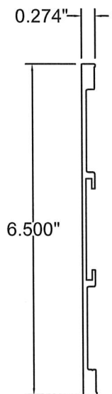
29 4" Surface Applied Muntin 6063-T6
