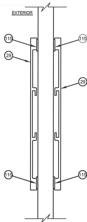
Section E-E 4" Surface Applied Muntin
