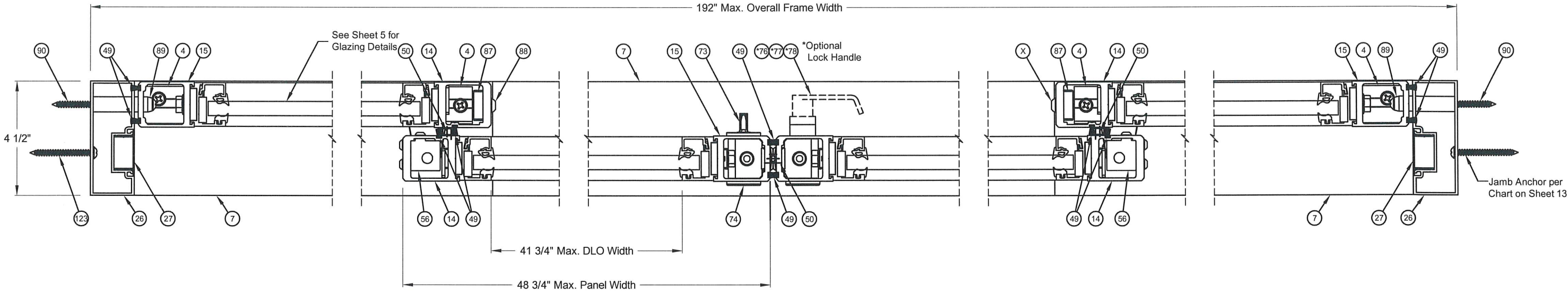
Section C-C, Narrow Stile BI-PARTING FIXED SIDELITE SHOWN
