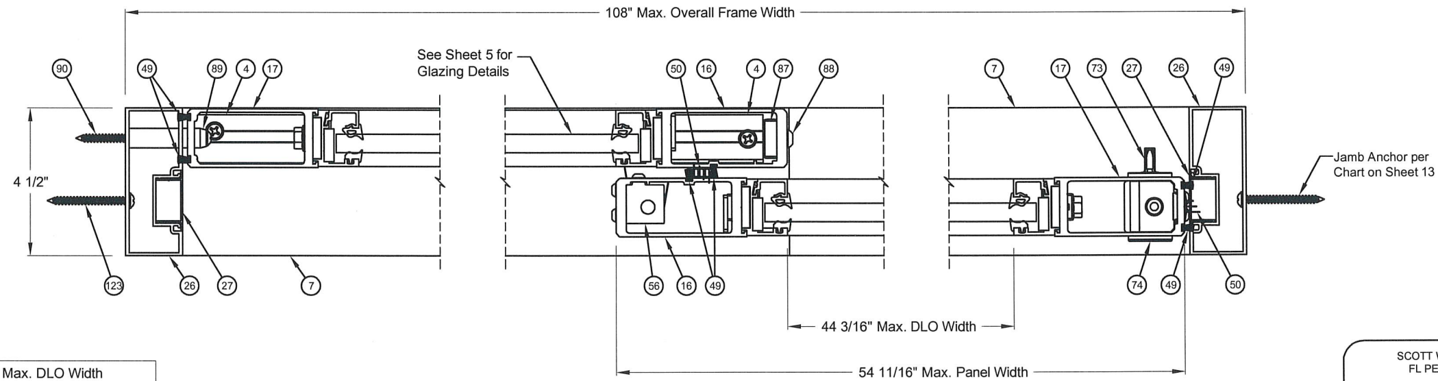
Section F-F, Medium Stile SINGLE SLIDE FIXED SIDELITE SHOWN
