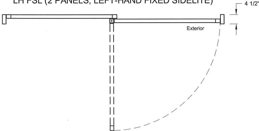
LH FSL (2 PANELS, LEFT-HAND FIXED SIDELITE)
