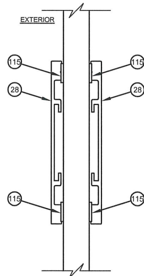
Section E-E 2" Surface Applied Muntin
