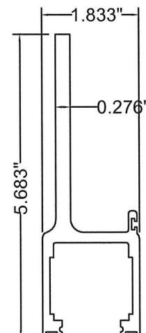
1 Carrier 6063-T6
