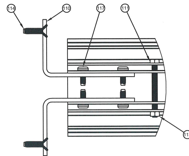
Section G-G True Divided 2" Muntin
