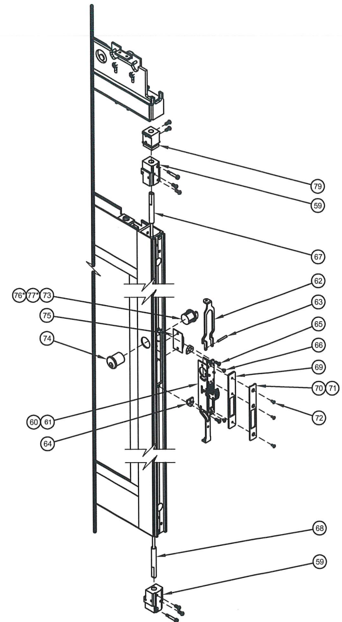
Locking System (Single Slide shown)
